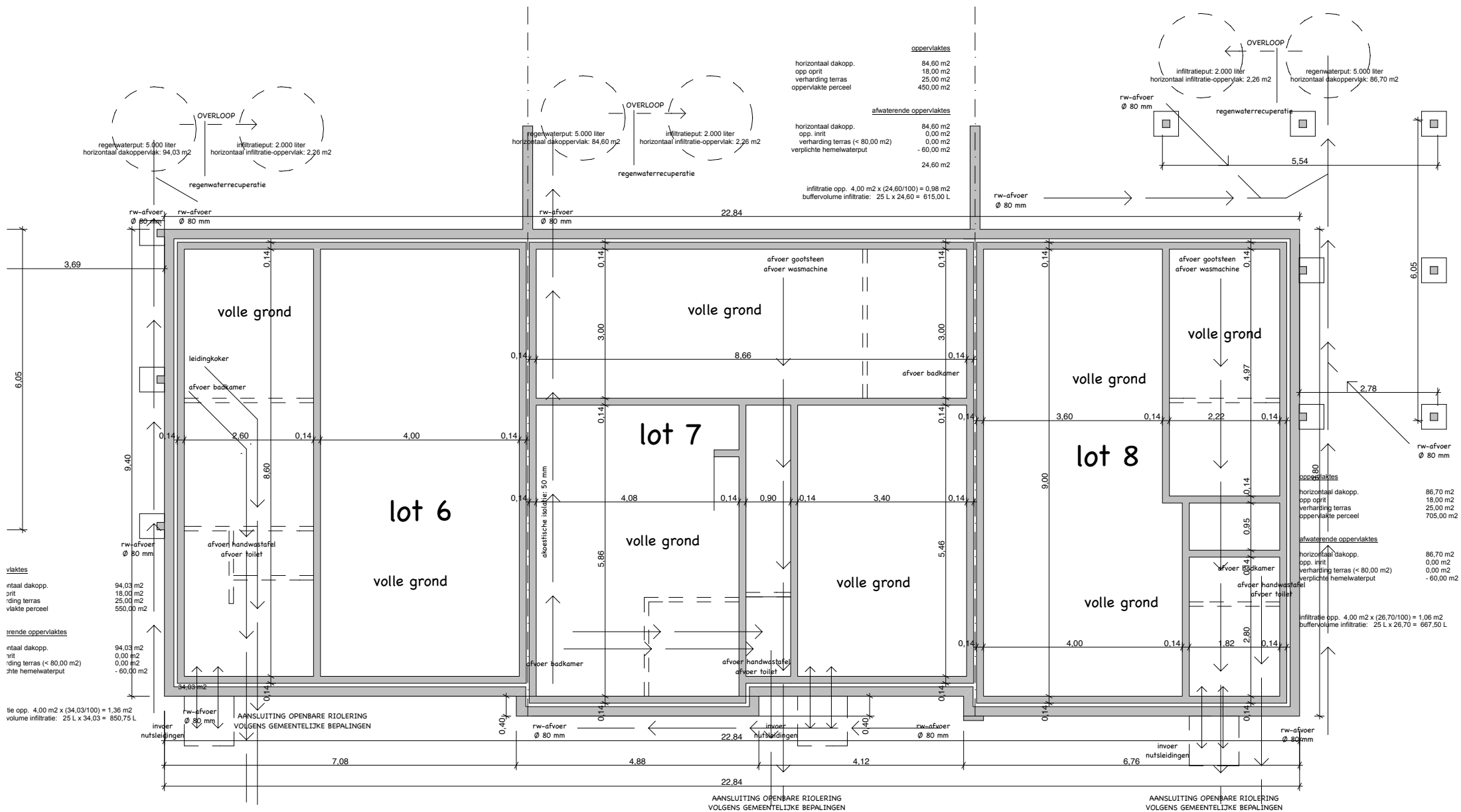
FUNDERINGS- en RIOLERINGSPLAN - lot 6 TEM 8 schaal: 1/100
