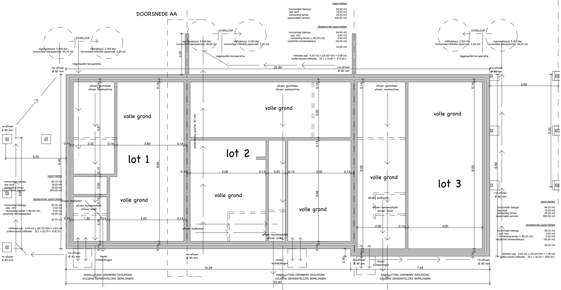
FUNDERINGS- en RIOLERINGSPLAN - lot 1 TEM 3 schaal: 1/100
