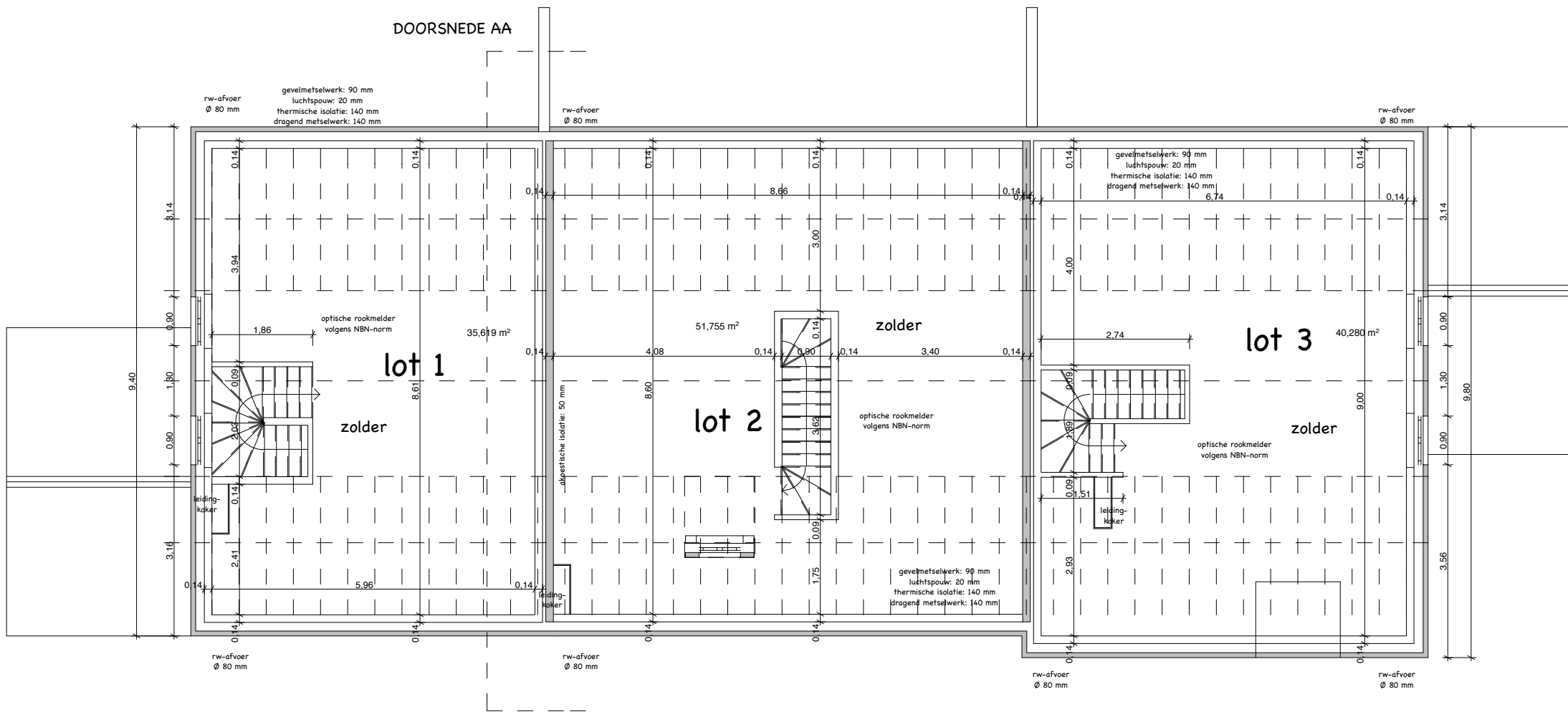
TWEEDE VERDIEPING - lot 1 TEM 3 schaal: 1/100
